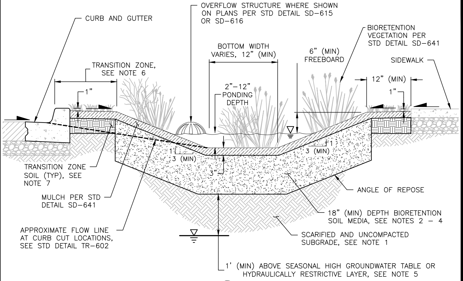
SECTION B NTS SD-611, TR-601
