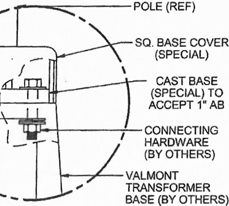
POLE AND BASE DETAIL - A
