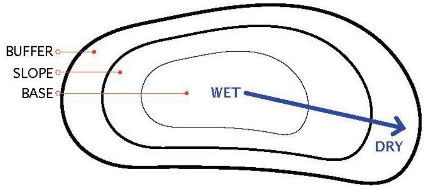
Fig. 4.30: Rain Garden Zones
